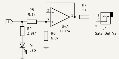
Output Stage (Repeat for 1, 2, 3 and 4 on all three channels)
