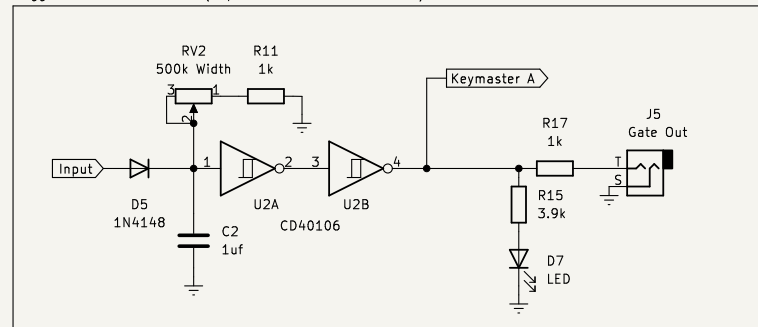
Trigger-to-Gate Converter (Repeat for Channels A, B & C)
