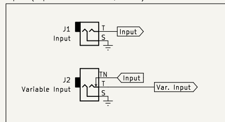
Inputs (Repeat for Channels A, B & C)
