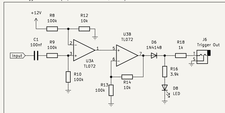
Gate-to-Trigger Converter (Repeat for Channels A, B & C)
