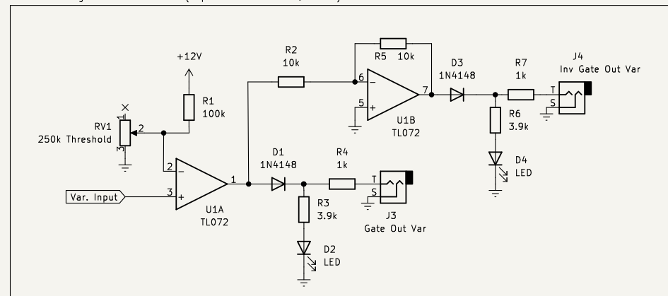
Variable Voltage to Gate Converter (Repeat for Channels A, B & C)
